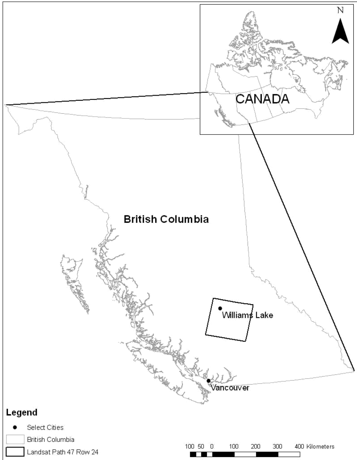
Figure 1: Map of the study area. The study site encompasses a Landsat scene (185 x 185 km 2 near Williams Lake BC, Canada
