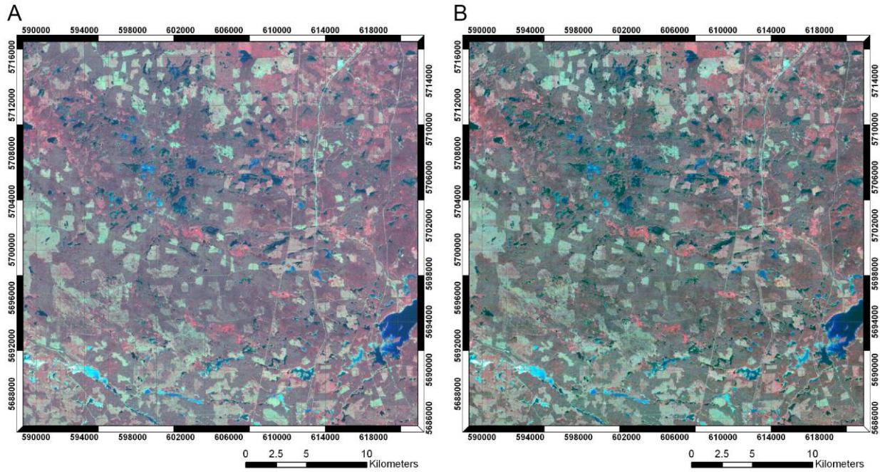
Figure 4: Comparison of fine scale structure between observed Landsat scene (acquired July 09 2008) and predicted Landsat scene (predicted using July 12 as prediction date). STARFM was able to represent the heterogeneity of Landscape well.
