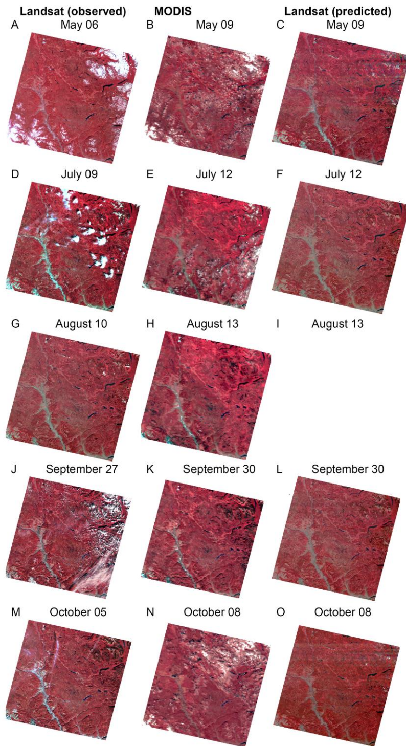
Figure 3: Comparison between observed Landsat scene (left column), observed MODIS scene (central column) and predicted Landsat scene (right column) for the 5 acquisition dates. No synthetic data has been predicted for August 13 as the Landsat input data from August have been used as T_1 image (Band combination: NIR, Red, Green).
