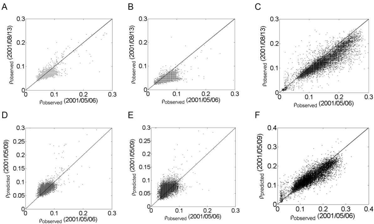
Figure 7 A-F: Capability of STARFM to predict seasonal changes in reflectance. Data include only those pixel values whose location coincided with vegetated land cover classes as defined by the EOSD maps. Figure 7A-C: Comparison between the Landsat TM reflectance observed at May 6 and the Landsat TM reflectance
