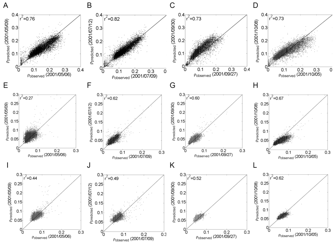
Figure 5: Per-pixel comparison between observed and predicted Landsat reflectance. The rows represent the reflectance values for the NIR, red and green TM band, respectively, the columns represent the four validation dates. Highest correlations between observed and predicted pixel values were found for the NIR band ( 0.73 < r^2 < 0.82 ; p < 0.01 ) (Figure 5A-D), while the visible reflectances yielded weaker relationships ( 0.27 < r^2 < 0.67 for the red (Figure 5E-H), and 0.44 < r^2 < 0.62 for the green band (Figure 5I-L)) ( p < 0.01 ). Prediction accuracy was highest for the scenes predicted for July 12 and September 30 (Figure 5B-C, F-G and J-K), while the accuracy was lower especially for the visible bands at the beginning of the vegetation period (Figure 5 E,I).
