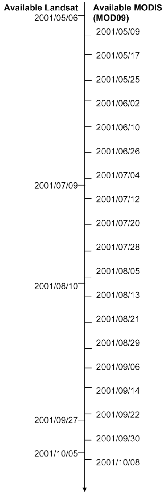
Figure 2: Acquisition dates of Landsat and MODIS scenes used for this study. Note that MODIS data were acquired as 8-day composites, the dates given in the figure are the first day of the 8-day acquisition period, respectively.
