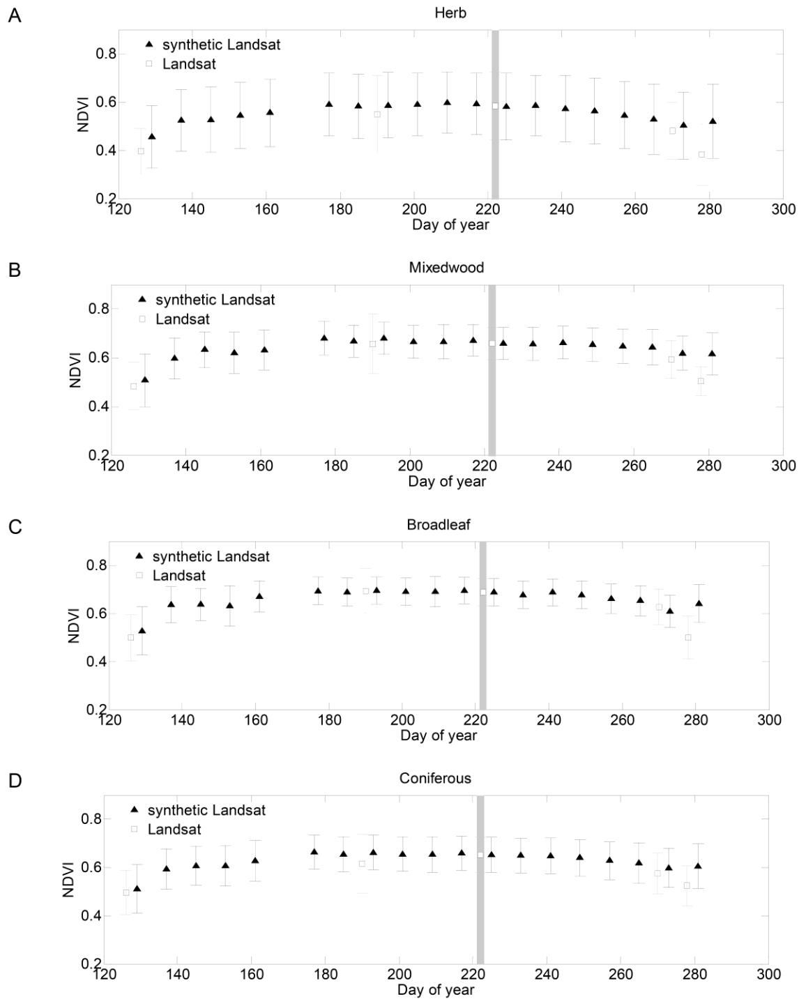
Figure 8: Eight-day time series of mean NDVI values calculated for the most common land cover types between DOY 120 to 280 (2001). The triangles show the mean NDVI values derived from STARFM synthetic images, the corresponding errorbars represent the standard deviation. The open squares mean NDVI values derived from the actual Landsat observations, the errorbars represent the standard deviation. The grey line at DOY 226 marks the T 1 date which was used for the STARFM predictions. Synthetic NDVI observations fit well into the annual pattern of the vegetation cycle for the different land cover types. Greatest differences in reflectance due to seasonal effects were found for the broadleaf vegetation class ( \Delta\text{NDVI}_{\text{max}}=0.21 ), while the coniferous land cover type maintained a more homogeneous level of NDVI ( \Delta\text{NDVI}_{\text{max}}=0.16 ).
