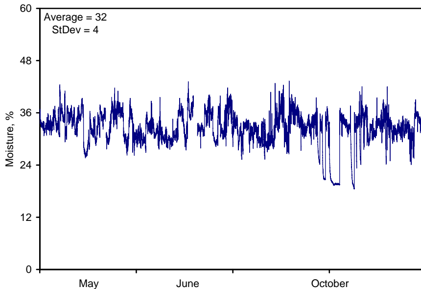
Figure 23. Chip moisture for all three periods
