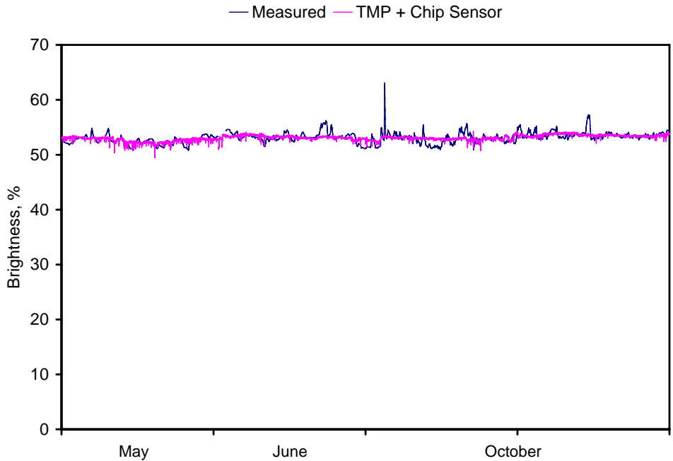
Figure 21. Measured and predicted brightness for all three periods combined using TMP operating variables and chip properties
