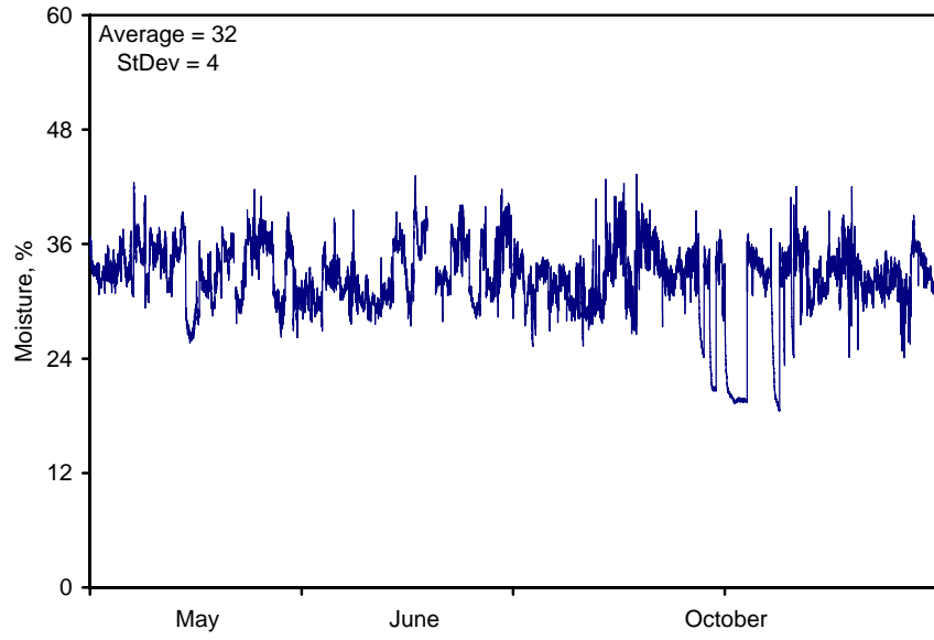
Figure 8. Chip moisture for all three periods.
