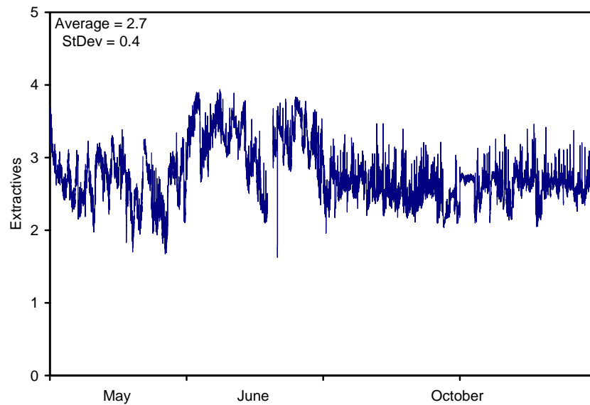
Figure 11. Chip extractives content for all three periods.
